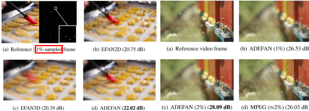
Fig 1: The sample reference frame is reconstructed from 1% randomly-sampled pixels (a), using different methods. (b) EFAN2D can track motion but causes disturbing video flickering. (c) EFAN3D achieves video stability at the cost of excessive temporal blurring effects. (d) Our adaptive ADEFAN method leverages the advantages of both (b) and (c). We achieve the best video reconstruction accuracy with minimal flickering.
