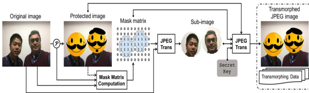
Figure1. Protection procedure of secure JPEG transmorphing
